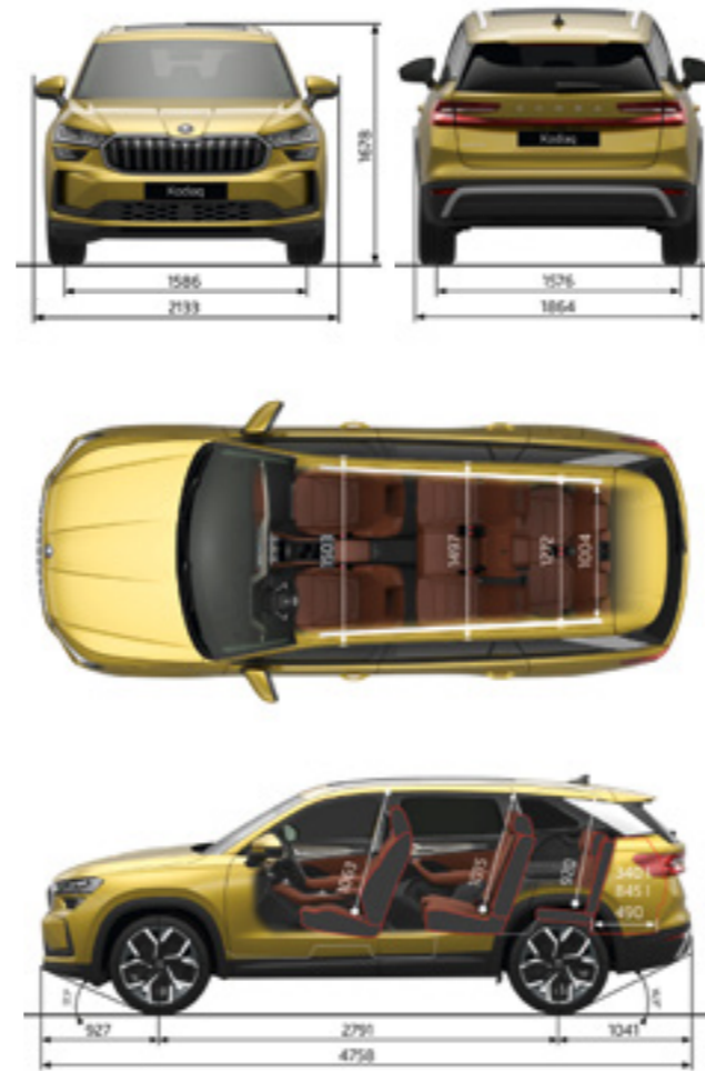
Dimensions (7-seat)
