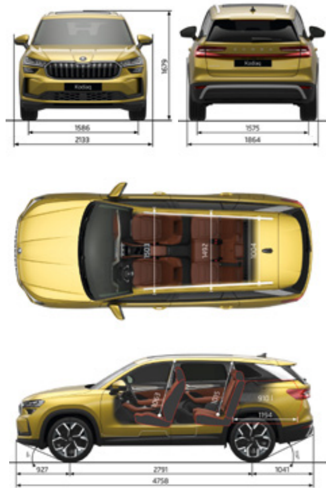
Dimensions (5-seat)
